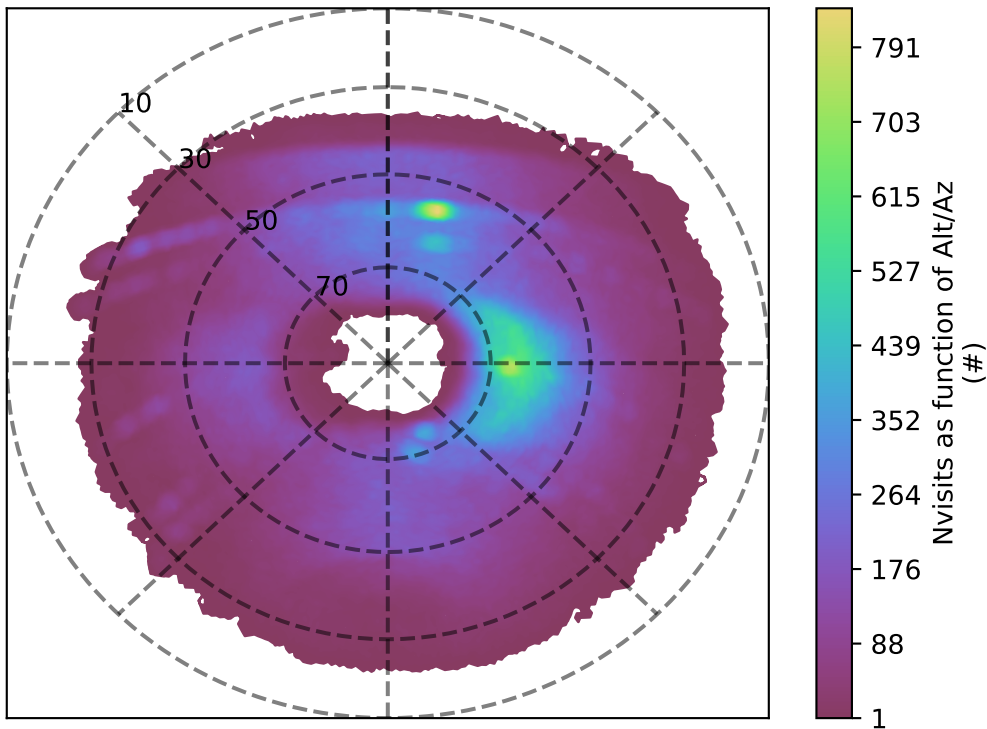
ddf_acor_sf10_lsf20_lsr20_v3.4_10yrs u band: Nvisits as function of Alt/Az
