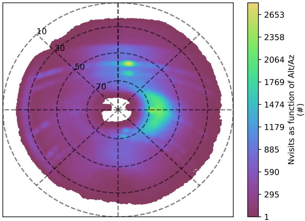
ddf_acor_sf10_lsf20_lsr20_v3.4_10yrs r band: Nvisits as function of Alt/Az
