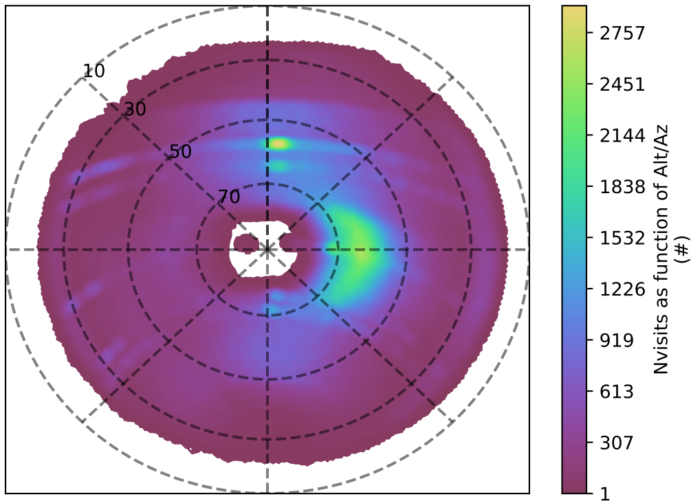
ddf_acor_sf10_lsf20_lsr20_v3.4_10yrs i band: Nvisits as function of Alt/Az
