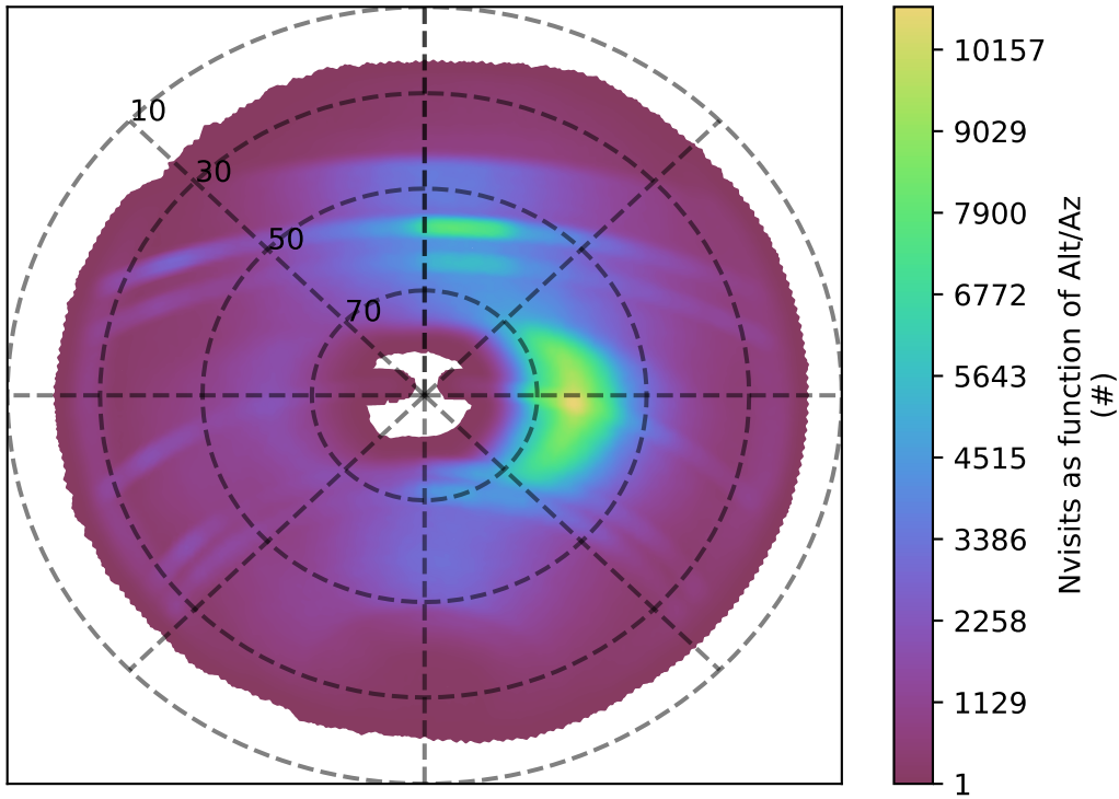
ddf_acor_sf10_lsf20_lsr20_v3.4_10yrs all bands: Nvisits as function of Alt/Az
