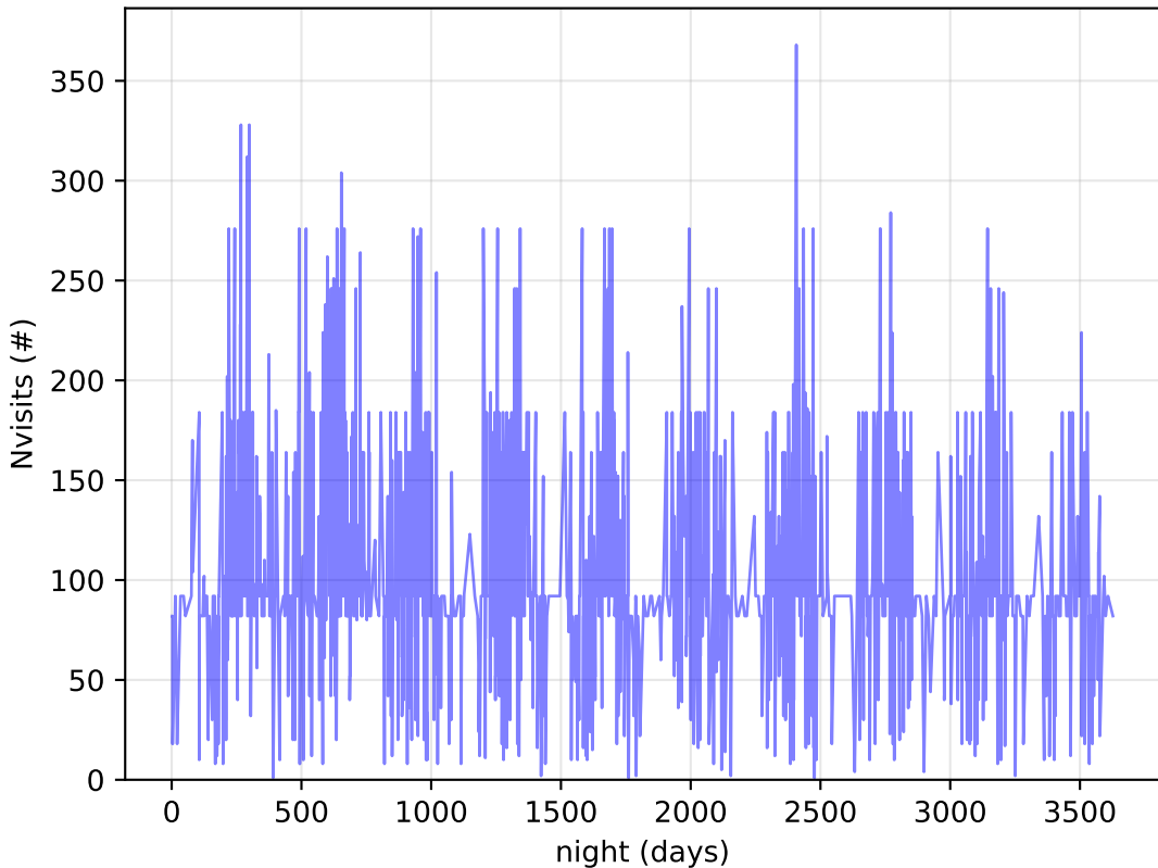
ddf_acor_sf10_ls20_lsr20_v3.4_10yrs DDF: Nvisits
