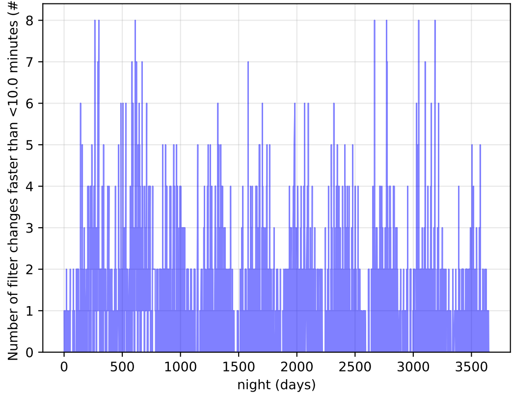
ddf_acor_sf10_Isf20_Isr20_v3.4_10yrs Per Night: Number of filter changes faster than <10.0 minutes
