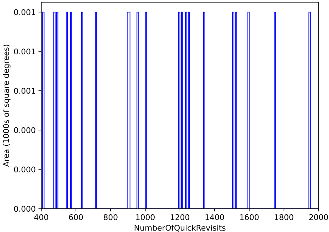
ddf_acor_sf10_lsf20_lsr20_v3.4_10yrs All sky: NumberOfQuickRevisits
