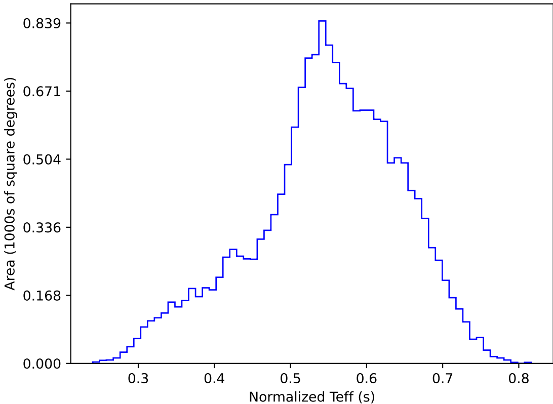
ddf_acor_sf10_lsf20_lsr20_v3.4_10yrs WFD y band: Normalized Teff
