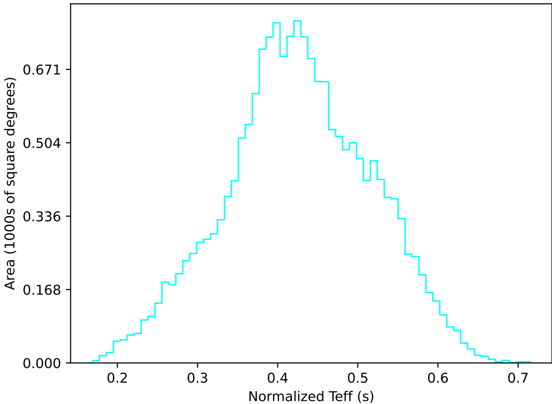
ddf_acor_sf10_lsf20_lsr20_v3.4_10yrs WFD u band: Normalized Teff
