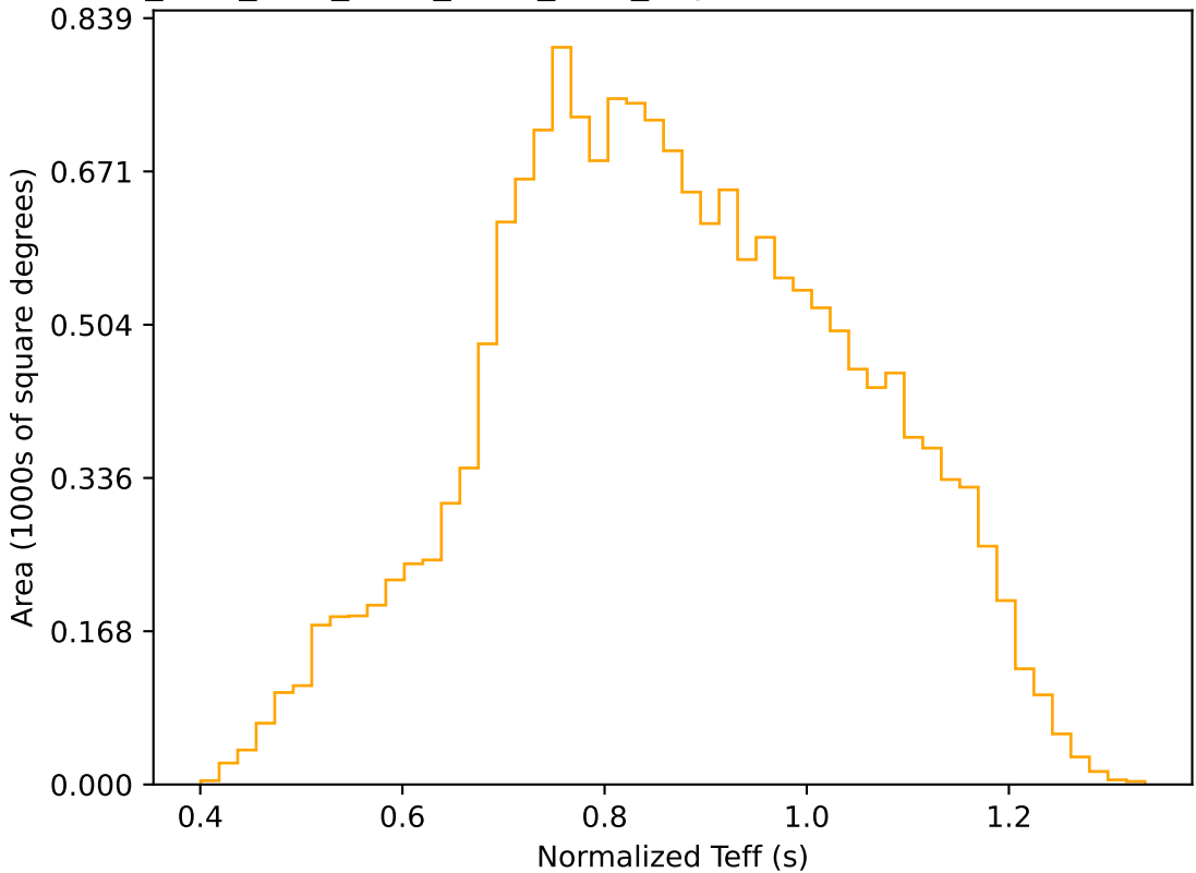
ddf_acor_sf10_lsf20_lsr20_v3.4_10yrs WFD r band: Normalized Teff
