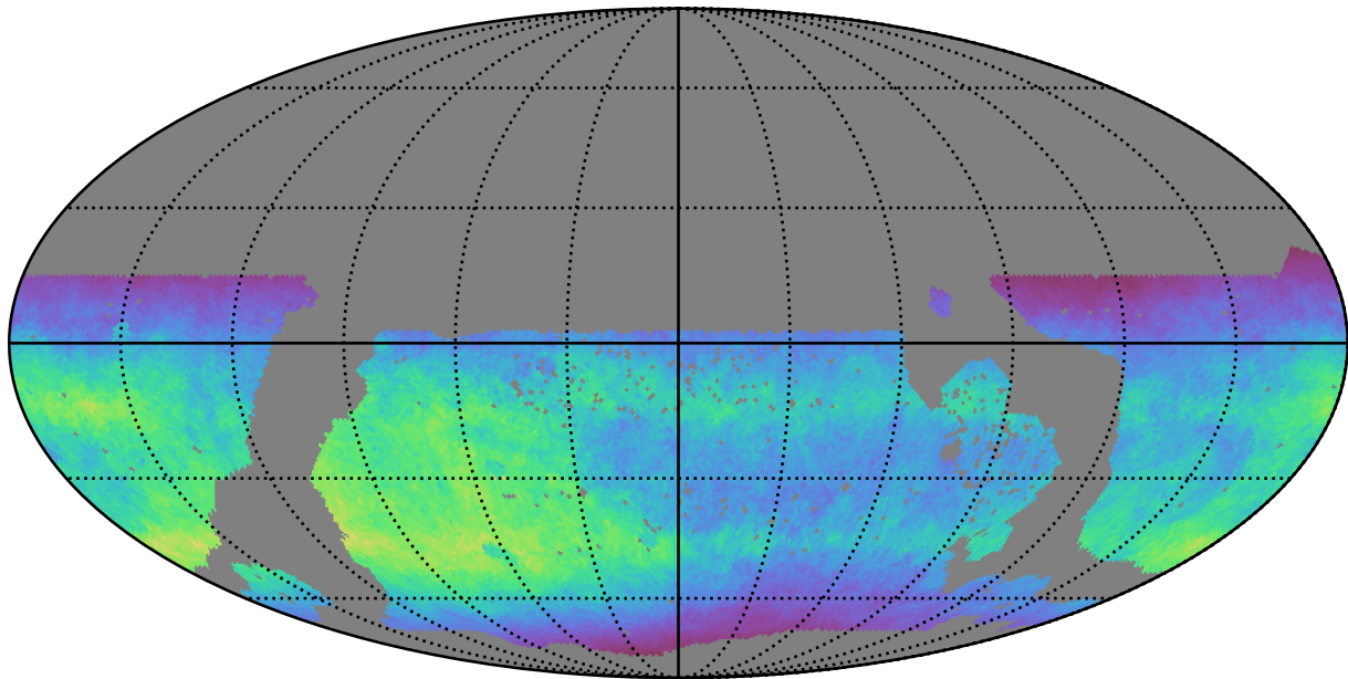
ddf_acor_sf10_lsf20_lsr20_v3.4_10yrs WFD i band: Normalized Teff
