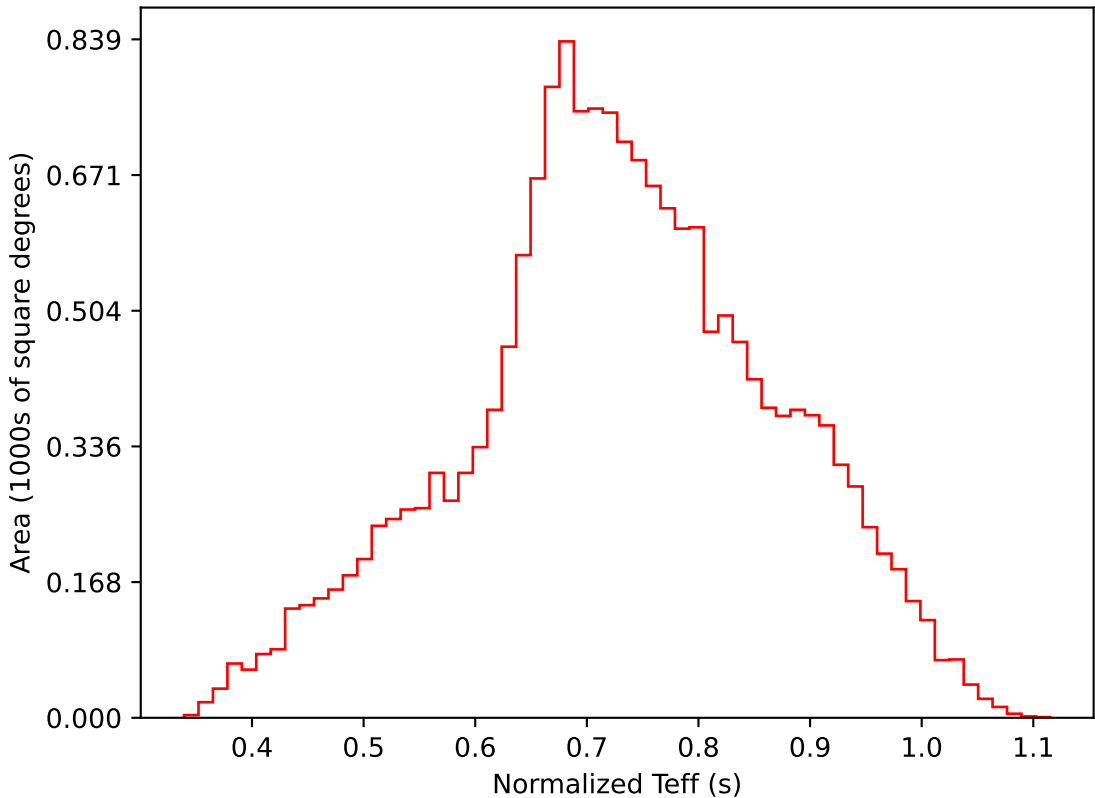
ddf_acor_sf10_lsf20_lsr20_v3.4_10yrs WFD i band: Normalized Teff
