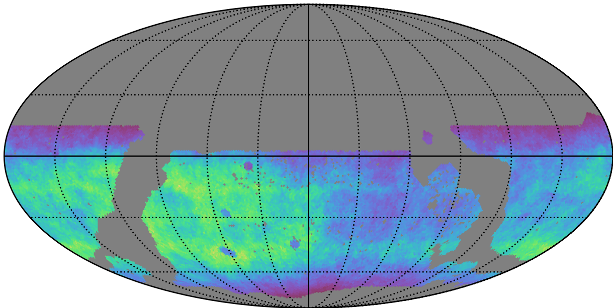
ddf_acor_sf10_lsf20_lsr20_v3.4_10yrs WFD g band: Normalized Teff
