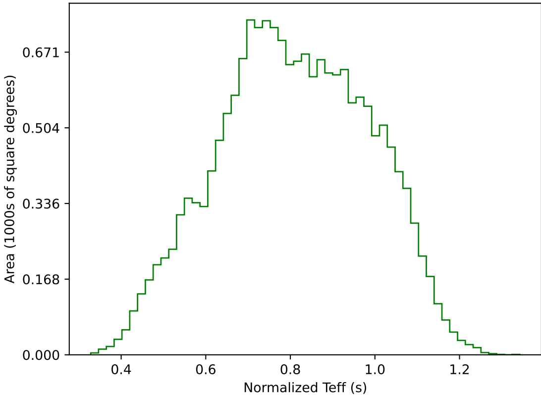
ddf_acor_sf10_lsf20_lsr20_v3.4_10yrs WFD g band: Normalized Teff
