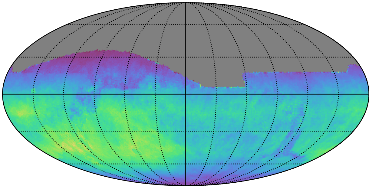
ddf_acor_sf10_lsf20_lsr20_v3.4_10yrs All sky z band: Normalized Teff
