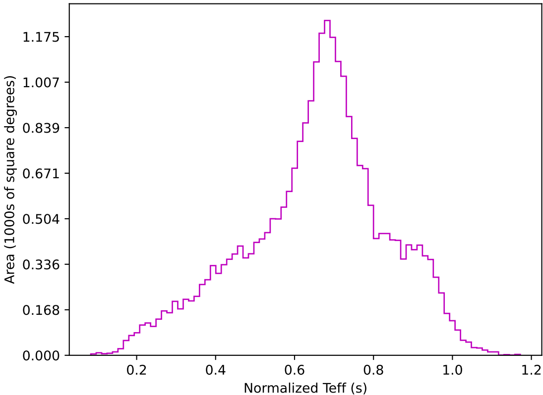
ddf_acor_sf10_lsf20_lsr20_v3.4_10yrs All sky z band: Normalized Teff
