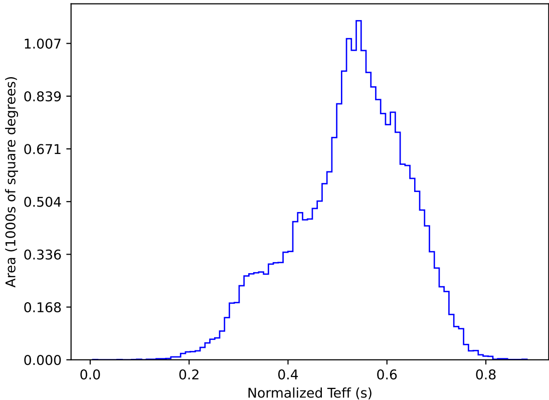
ddf_acor_sf10_lsf20_lsr20_v3.4_10yrs All sky y band: Normalized Teff
