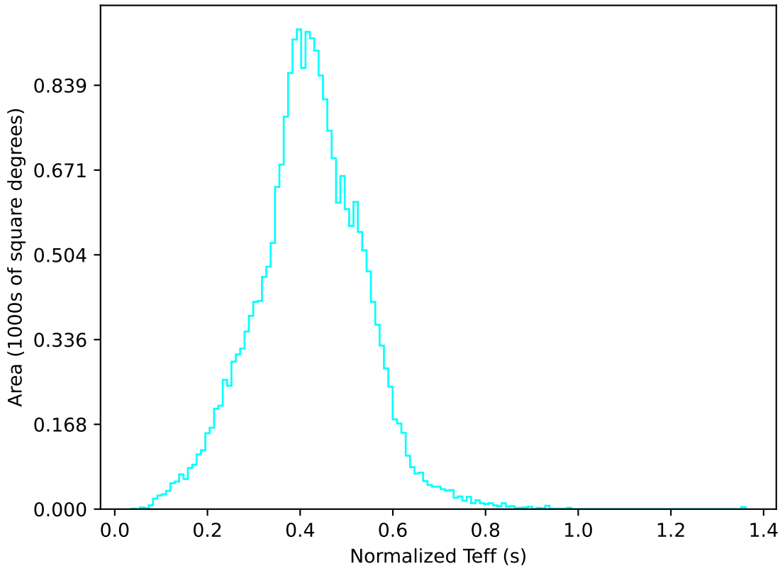
ddf_acor_sf10_lsf20_lsr20_v3.4_10yrs All sky u band: Normalized Teff
