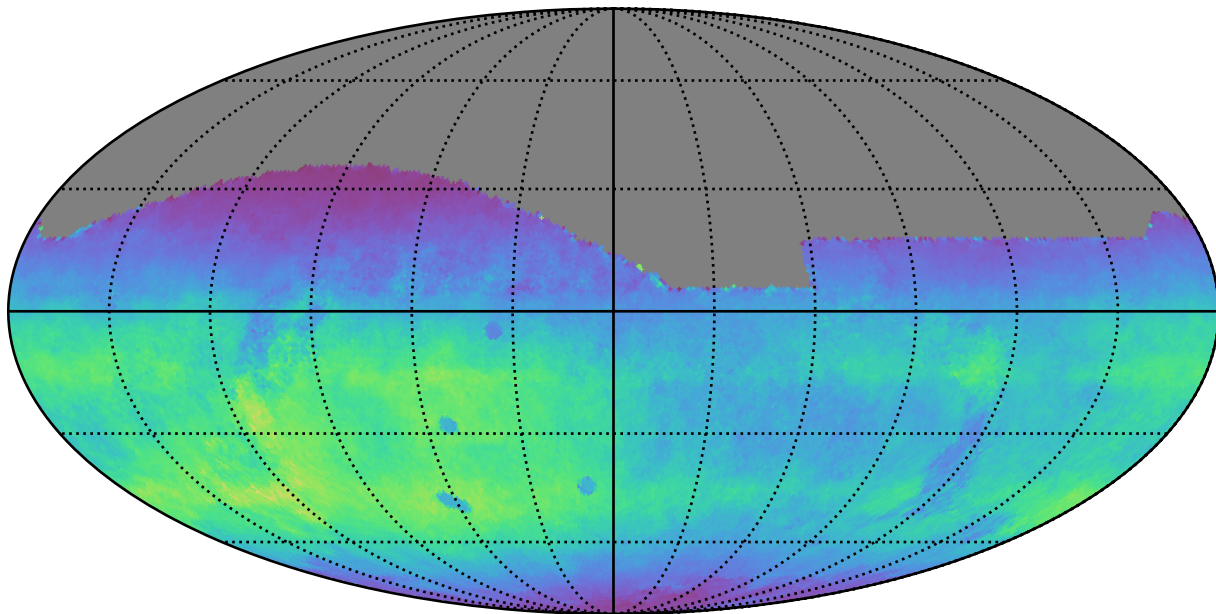
ddf_acor_sf10_lsf20_lsr20_v3.4_10yrs All sky r band: Normalized Teff
