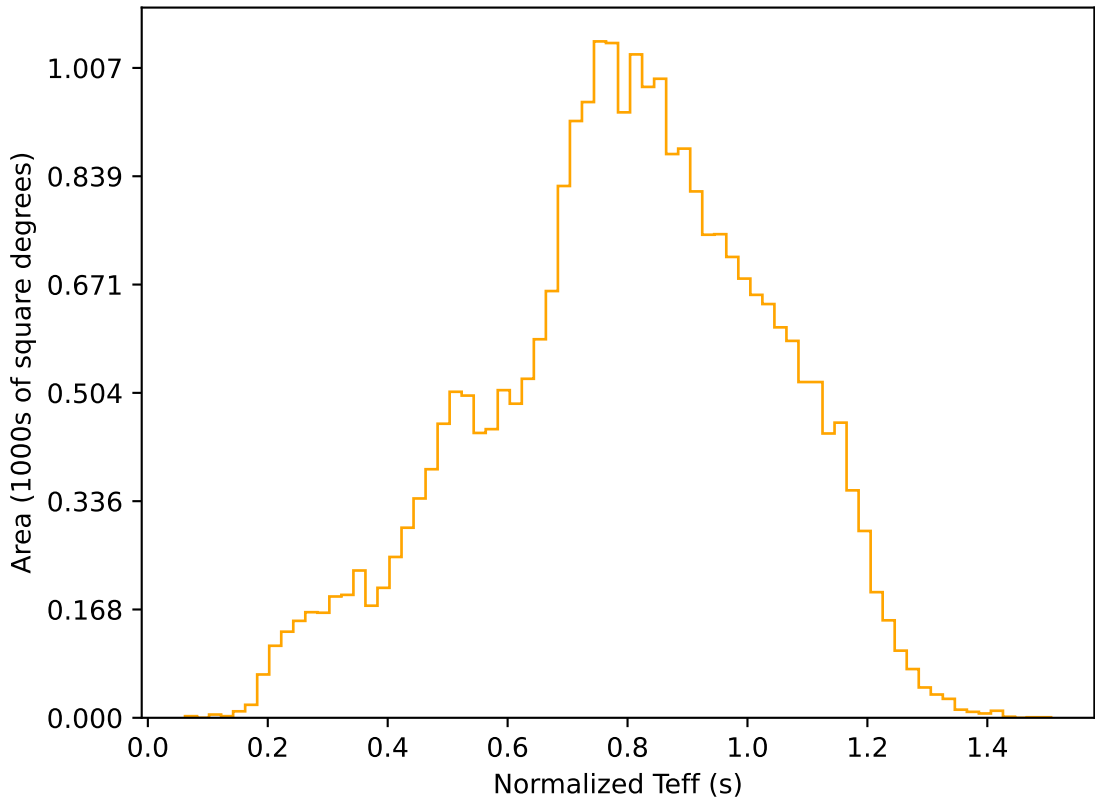
ddf_acor_sf10_lsf20_lsr20_v3.4_10yrs All sky r band: Normalized Teff
