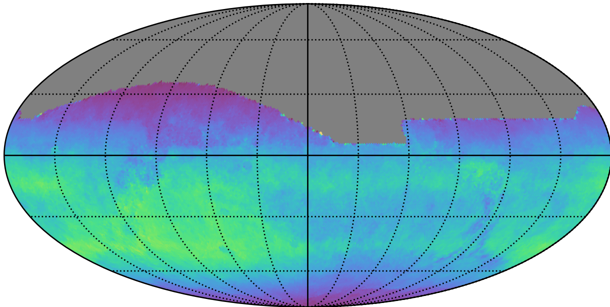
ddf_acor_sf10_lsf20_lsr20_v3.4_10yrs All sky i band: Normalized Teff
