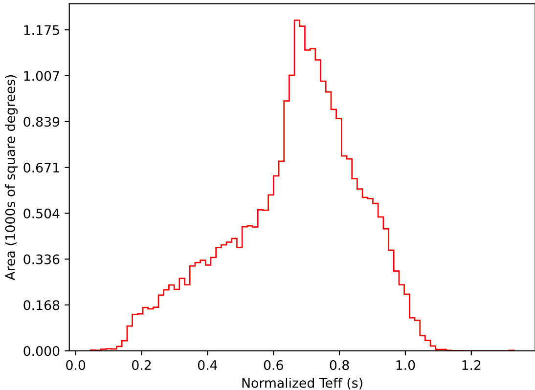
ddf_acor_sf10_lsf20_lsr20_v3.4_10yrs All sky i band: Normalized Teff
