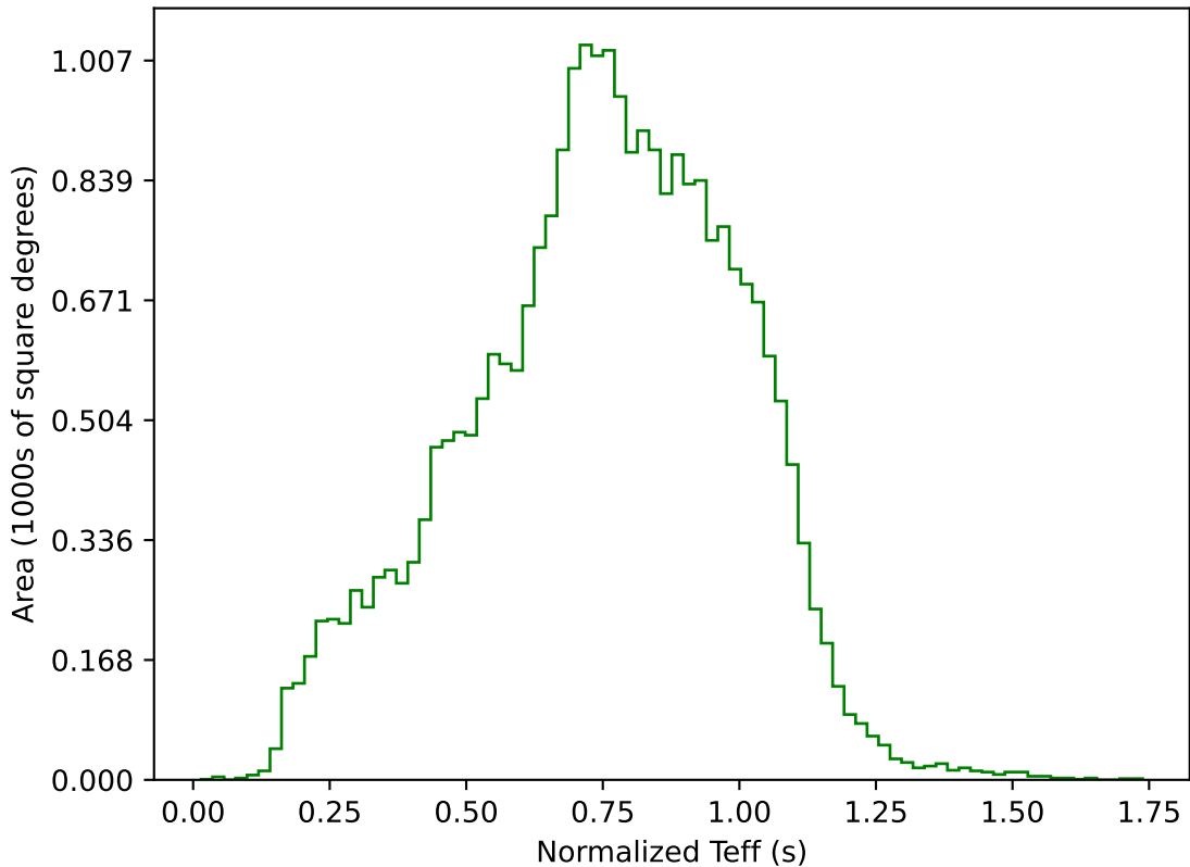
ddf_acor_sf10_lsf20_lsr20_v3.4_10yrs All sky g band: Normalized Teff
