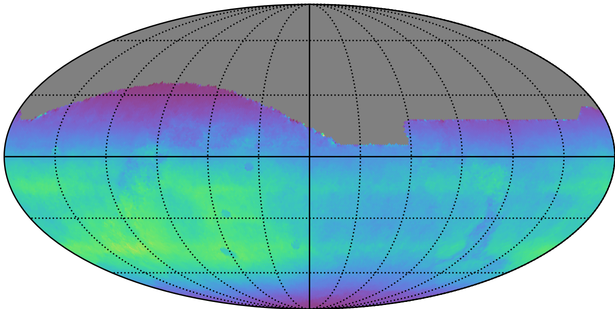
ddf_acor_sf10_lsf20_lsr20_v3.4_10yrs All sky all bands: Normalized Teff
