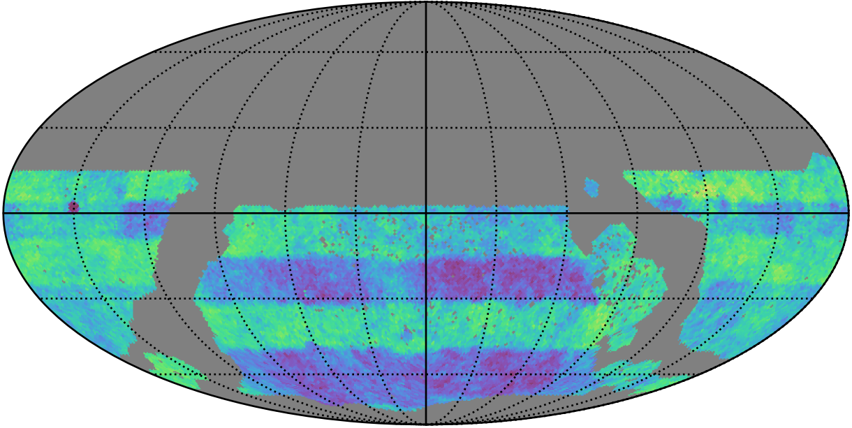
ddf_acor_sf10_lsf20_lsr20_v3.4_10yrs WFD: Normalized Proper Motion Uncert @ 24.0
