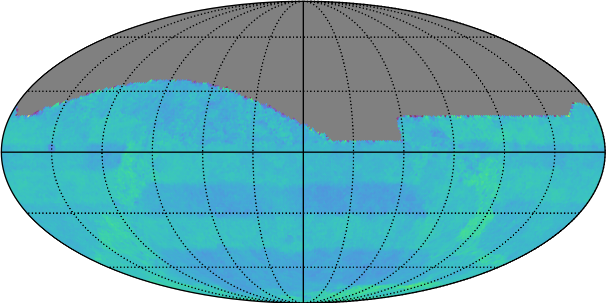
ddf_acor_sf10_lsf20_lsr20_v3.4_10yrs All sky: Normalized Proper Motion Uncert @ 24.0
