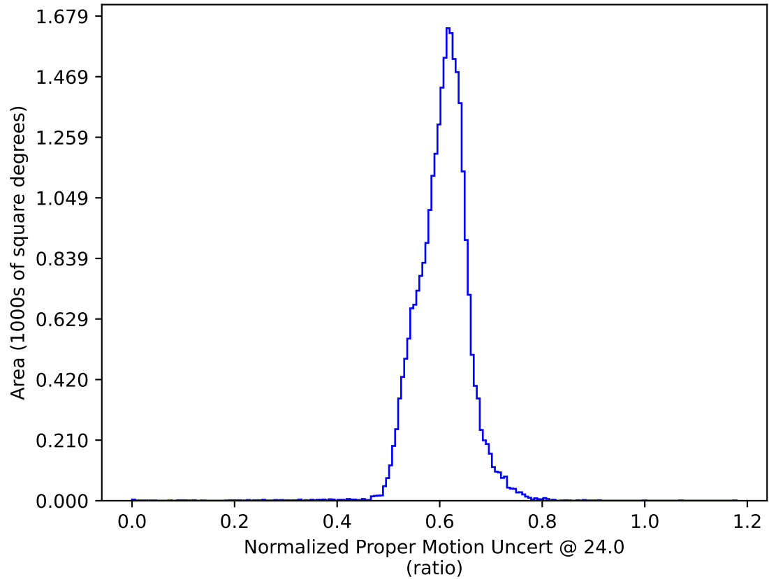
ddf_acor_sf10_lsf20_lsr20_v3.4_10yrs All sky: Normalized Proper Motion Uncert @ 24.0
