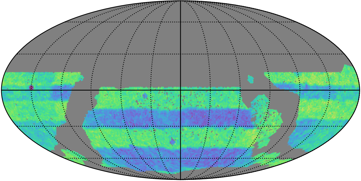
ddf_acor_sf10_lsf20_lsr20_v3.4_10yrs WFD: Normalized Proper Motion Uncert @ 20.5
