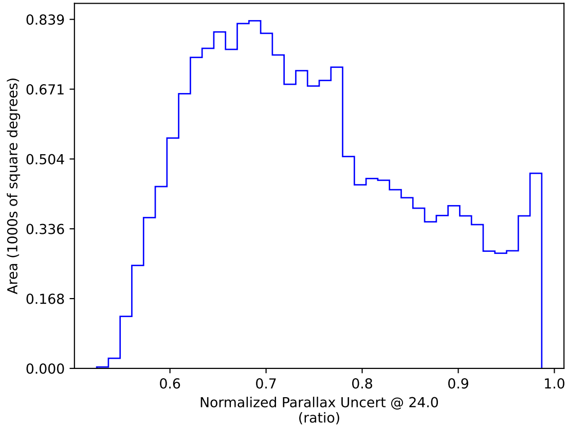
ddf_acor_sf10_lsf20_lsr20_v3.4_10yrs WFD: Normalized Parallax Uncert @ 24.0
