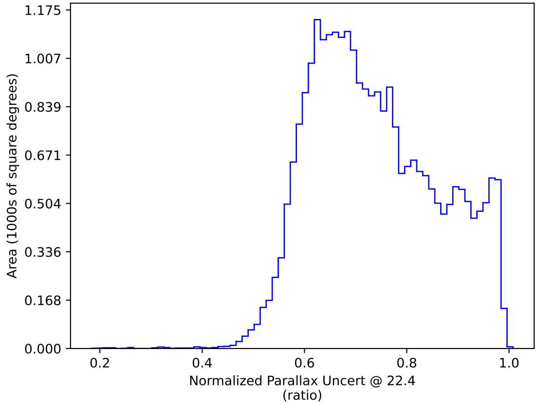
ddf_acor_sf10_lsf20_lsr20_v3.4_10yrs All sky: Normalized Parallax Uncert @ 22.4
