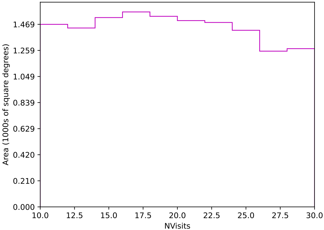
ddf_acor_sf10_lsf20_lsr20_v3.4_10yrs Yr 3-4 z band: NVisits
