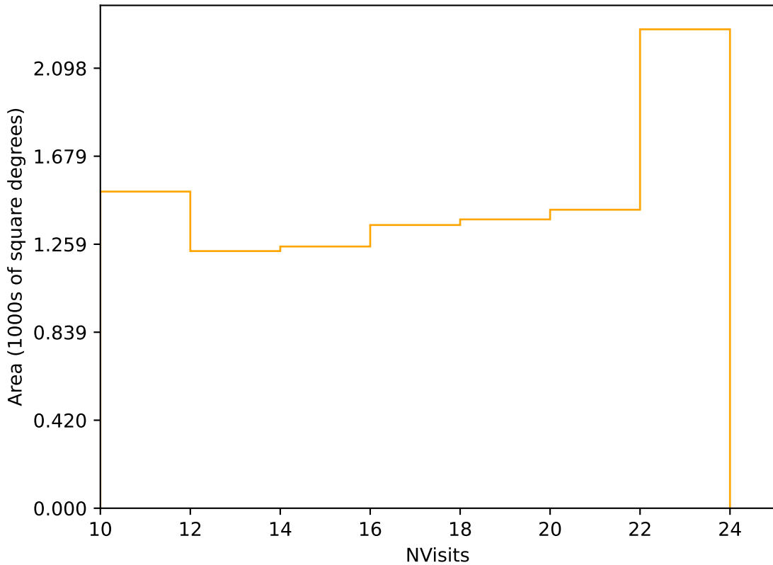
ddf_acor_sf10_lsf20_lsr20_v3.4_10yrs Yr 3-4 r band: NVisits
