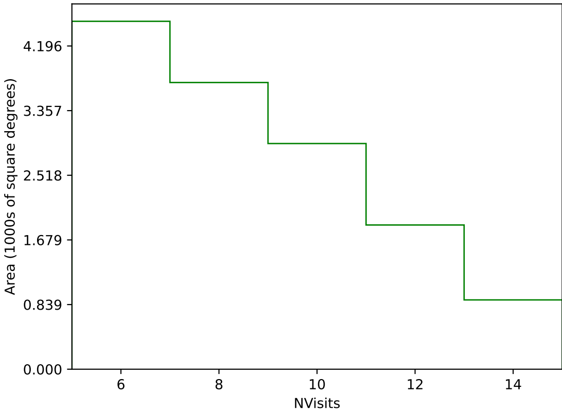
ddf_acor_sf10_lsf20_lsr20_v3.4_10yrs Yr 3-4 g band: NVisits
