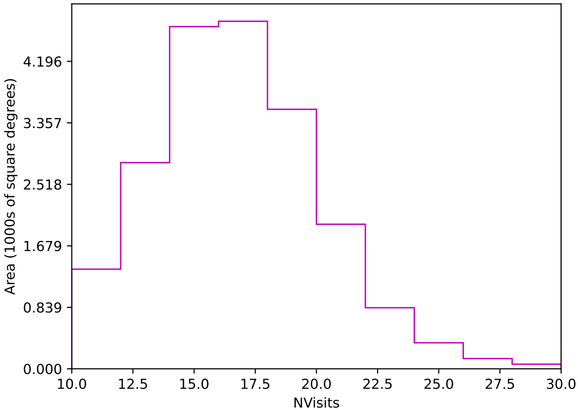
ddf_acor_sf10_lsf20_lsr20_v3.4_10yrs Yr 1 z band: NVisits
