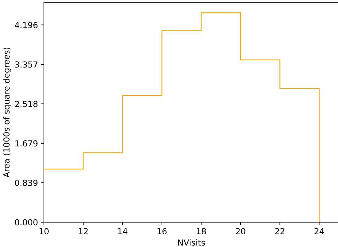
ddf_acor_sf10_lsf20_lsr20_v3.4_10yrs Yr 1 r band: NVisits
