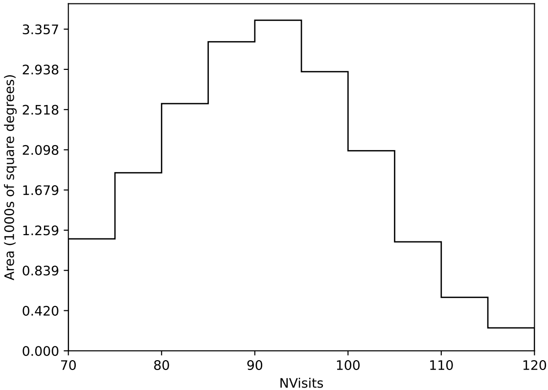
ddf_acor_sf10_lsf20_lsr20_v3.4_10yrs Yr 1 all bands: NVisits
