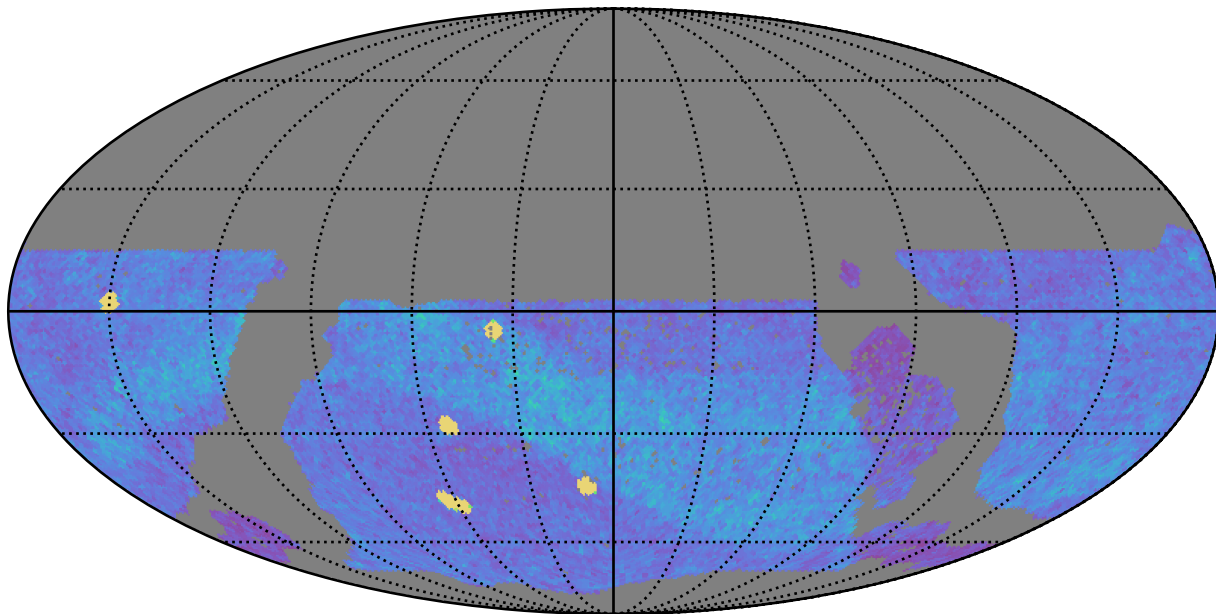
ddf_acor_sf10_lsf20_lsr20_v3.4_10yrs WFD z band: NVisits
