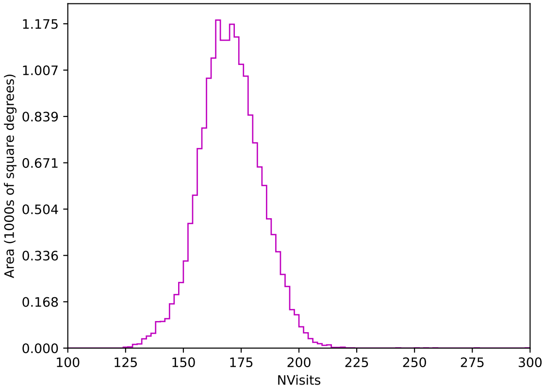
ddf_acor_sf10_lsf20_lsr20_v3.4_10yrs WFD z band: NVisits
