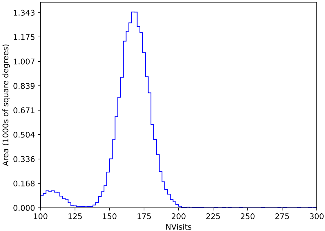
ddf_acor_sf10_lsf20_lsr20_v3.4_10yrs WFD y band: NVisits
