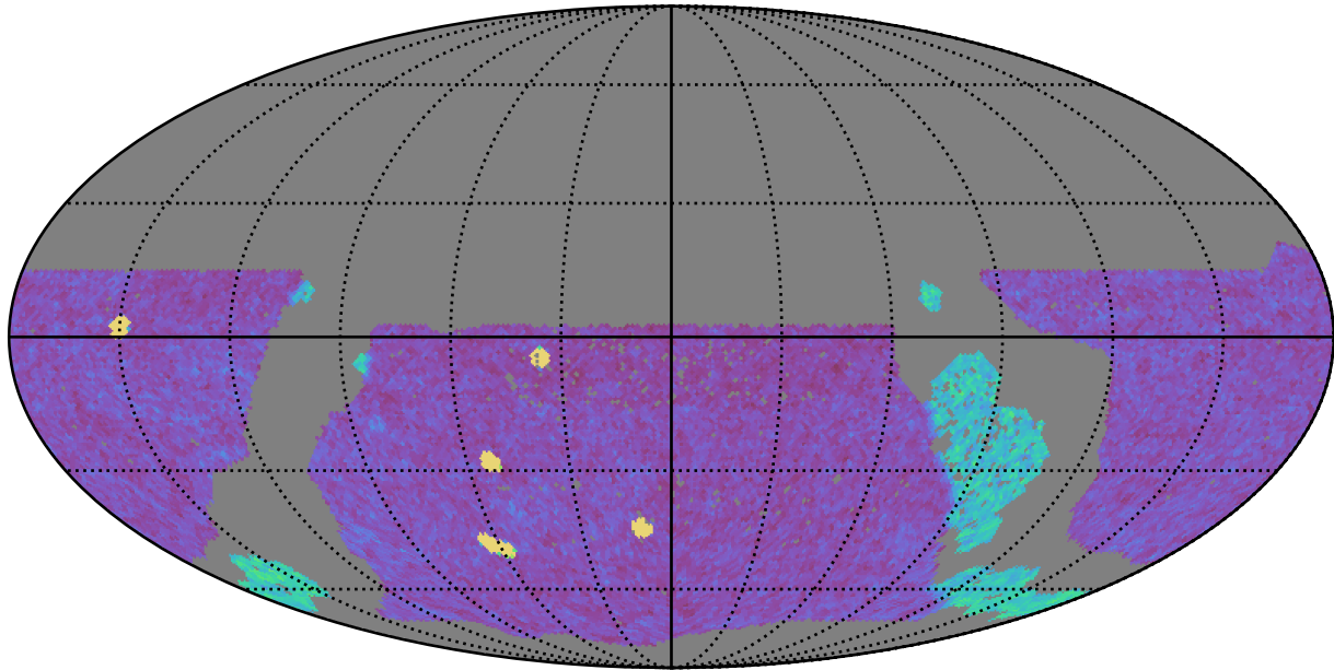
ddf_acor_sf10_lsf20_lsr20_v3.4_10yrs WFD g band: NVisits
