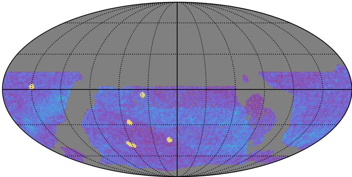
ddf_acor_sf10_lsf20_lsr20_v3.4_10yrs WFD all bands: NVisits
