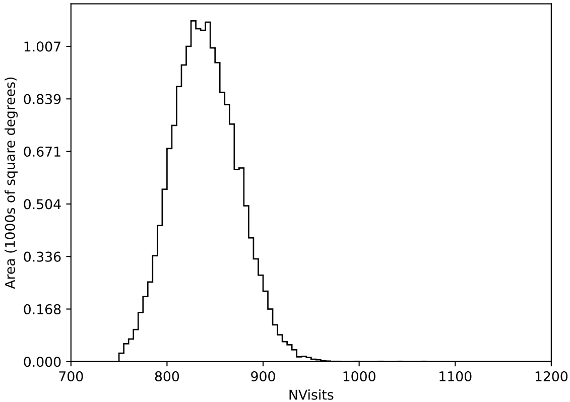
ddf_acor_sf10_lsf20_lsr20_v3.4_10yrs WFD all bands: NVisits
