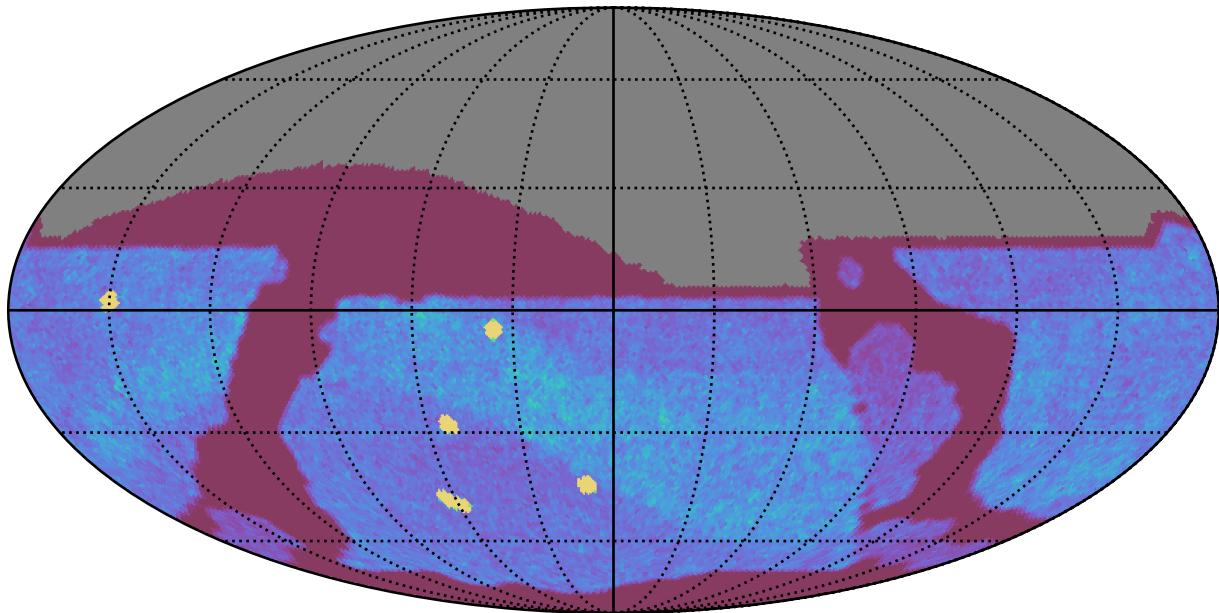
ddf_acor_sf10_lsf20_lsr20_v3.4_10yrs All sky z band: NVisits
