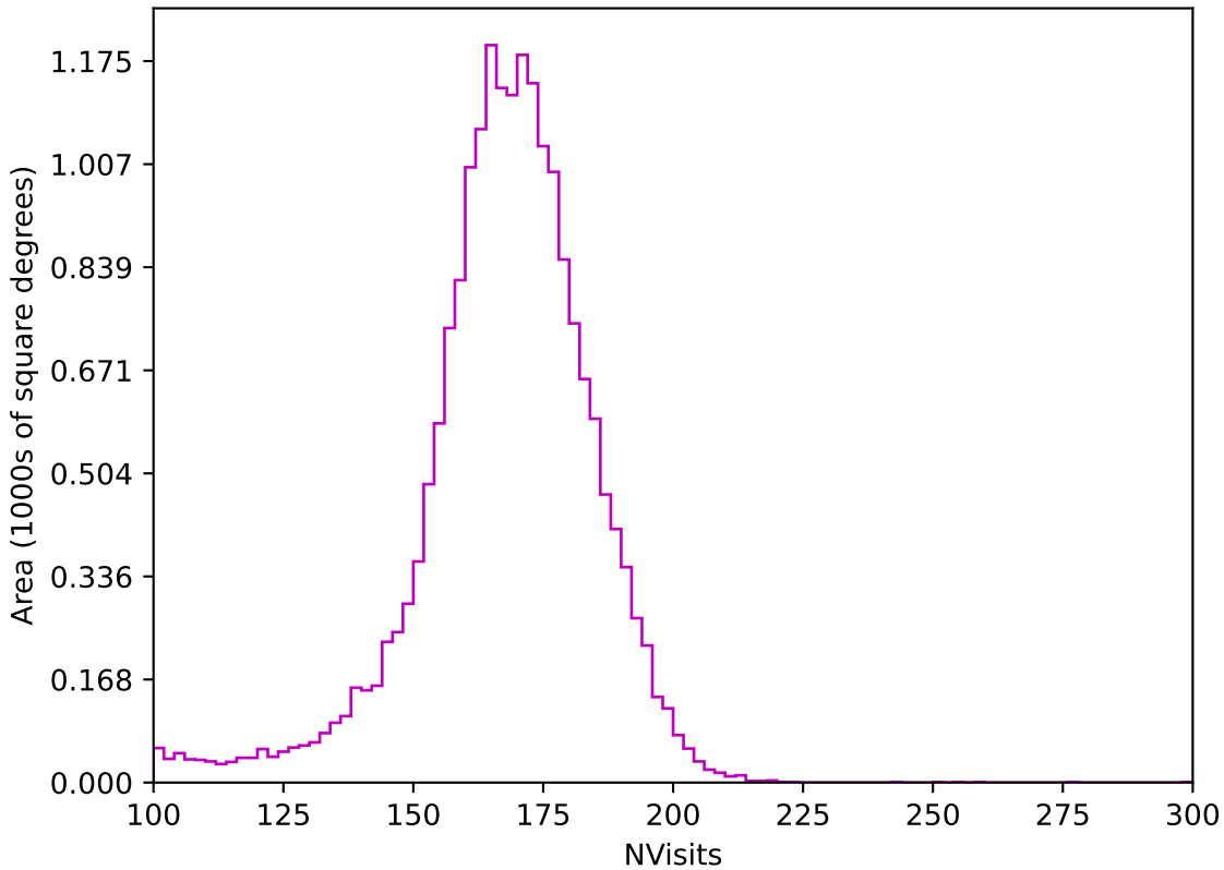
ddf_acor_sf10_lsf20_lsr20_v3.4_10yrs All sky z band: NVisits
