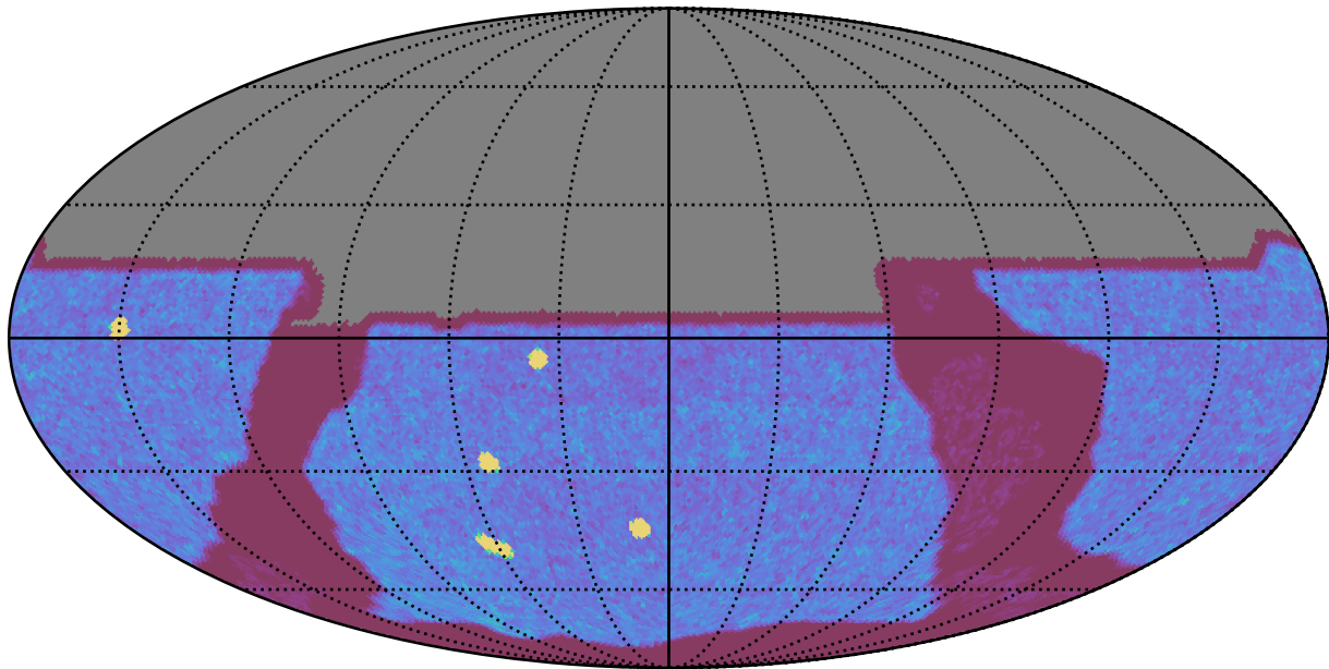
ddf_acor_sf10_lsf20_lsr20_v3.4_10yrs All sky y band: NVisits
