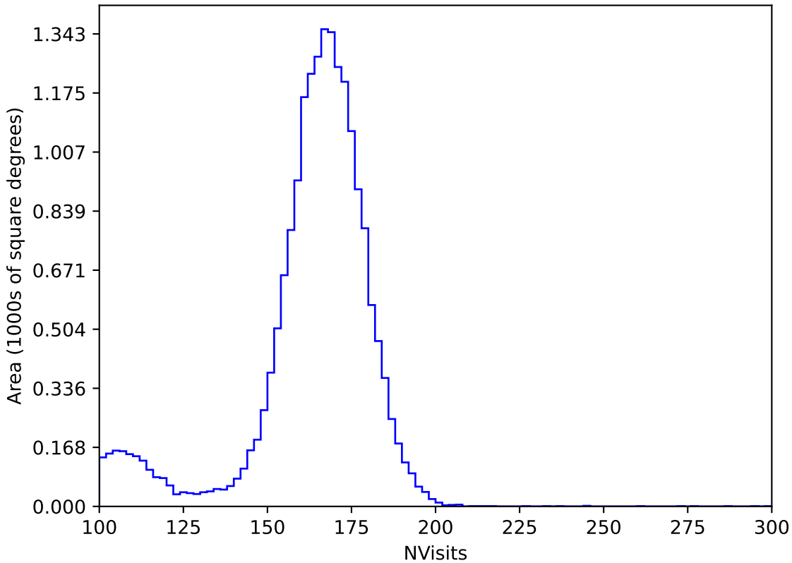
ddf_acor_sf10_lsf20_lsr20_v3.4_10yrs All sky y band: NVisits
