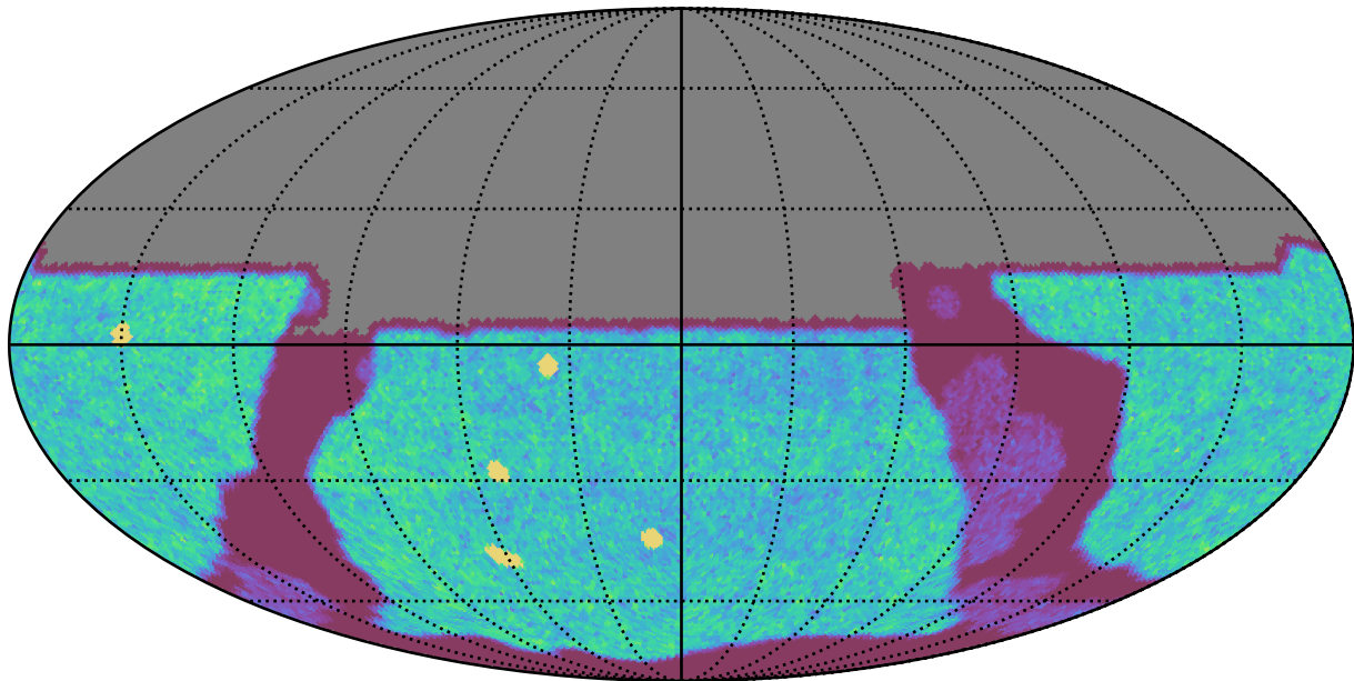
ddf_acor_sf10_lsf20_lsr20_v3.4_10yrs All sky u band: NVisits
