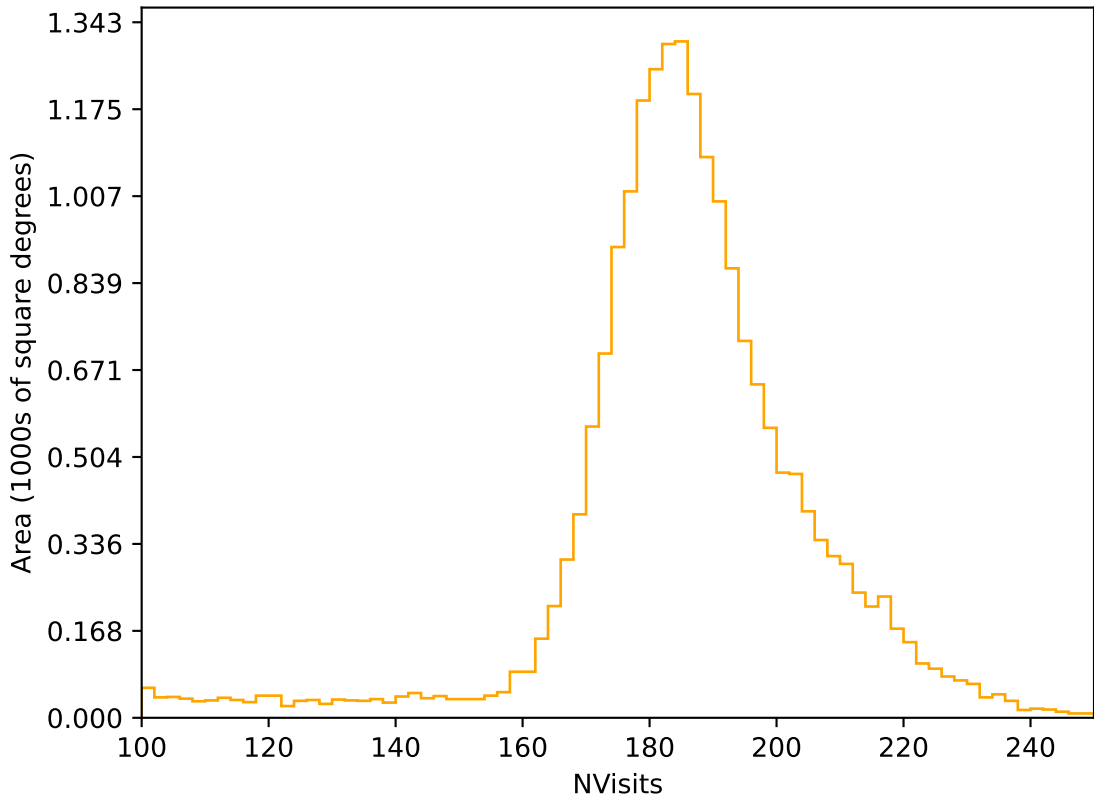
ddf_acor_sf10_lsf20_lsr20_v3.4_10yrs All sky r band: NVisits
