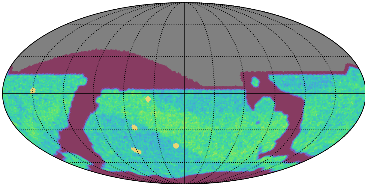
ddf_acor_sf10_lsf20_lsr20_v3.4_10yrs All sky i band: NVisits
