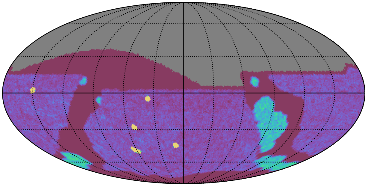
ddf_acor_sf10_lsf20_lsr20_v3.4_10yrs All sky g band: NVisits
